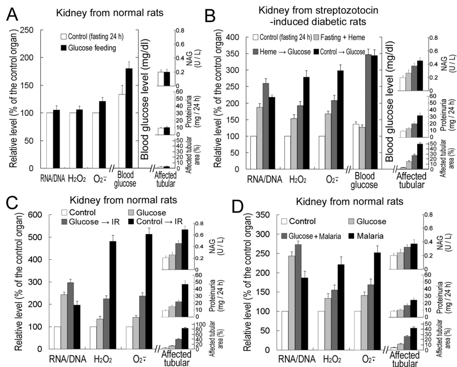
Figure 5. The role of RNA amplification in diabetes/IR/malaria-induced oxidative stress resistance of rat kidney cells. Kidney RNA/DNA ratio, H_2O_2 and superoxide levels and tubular damages (tubular dilation area (Figure SM-4), proteinuria level and N -acetyl- \beta glucosaminidase (NAG) level) and blood glucose levels in normal (A, C, D) and diabetic rats (B) were determined. The rat (fasted for 24 h for the “control” sample to diabetic experiments) kidneys were treated with or without 1 mmol/L heme or 30% glucose (renal arterial infusion), and then 30% glucose solution (every 8 h, 3× total) was administered orally or IR or malaria infection was performed. Samples were taken at 24 h after IR or glucose administration, or 8 d after malaria infection. The sample “glucose” means four times glucose infusion (every 2 d) without malaria infection. See “Materials and Methods” for details. Data in control samples are normalized to 100%. Error bars show standard deviations ( n = 3 ).
