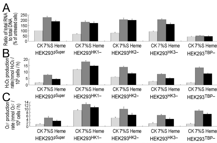
Figure 4. Effects of 7% glucose (7%S) and 50 μmol/L heme treatments (8 h) on total RNA levels (A), H 2 O 2 (B) and superoxide (C) production rates of HEK293 HK1- , HEK293 HK2- , HEK293 HK3- and HEK293 TBP- gene-silenced cell lines and the HEK293 pSuper control cell lines. CK, untreated control cells. Error bars show standard deviations (n = 3).
