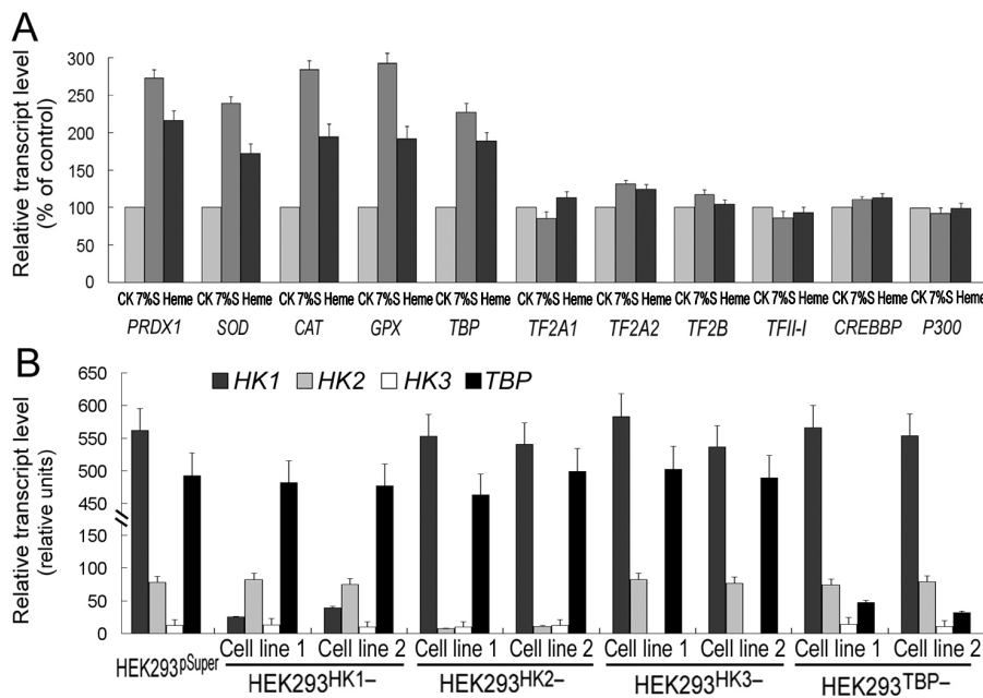
Figure 3. Representative gene expression in control or silenced HEK293 cell lines. (A) The 7% glucose (7%S) and 50 μmol/L heme increase PRDX1 , SOD , CAT , GPX and TBP expression but have no effect on the other six representative transcription factor genes in HEK293 cells. The treatment time was 24 h. Gene expression levels of the cells without any treatment (CK) are normalized to 100%. (B) HK1 , HK2 , HK3 and TBP expression levels in HEK293 HK1- , HEK293 HK2- , HEK293 HK3- and HEK293 TBP- gene-silenced cell lines and the HEK293 pSuper control cell lines. Two independent gene-silenced cell lines for each gene were tested. Gene expression levels were detected by quantitative real-time PCR. Gene-expressing detection was performed with Actin1 transcript as a loading control. Error bars show standard deviations (n = 3).
