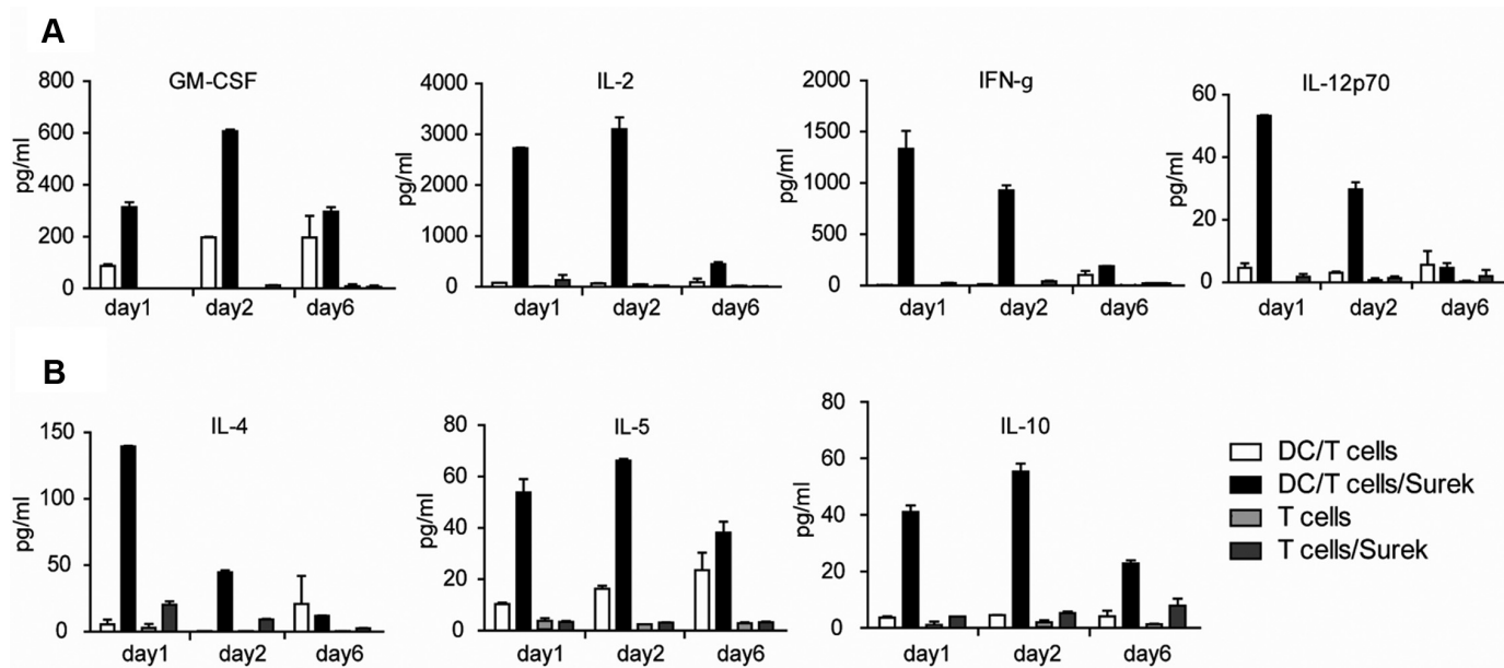
Figure 2. Cytokine patterns in cocultures containing T cells, DCs and Surek. After coculturing B78-D14 cells with DCs and T cells with or without 20 \mu\text{g}/\text{mL} Surek, cytokine levels were analyzed by using the Bioplex™ system. All groups contained B78-D14 cells. T cells, DCs and Surek were added as indicated. Supernatants were collected at d 1, 2 and 6. Means and standard deviations from three experiments are shown. (A) Th1-related cytokines GM-CSF, IL-2, IFN- \gamma and IL-12p70 in culture supernatants. (B) Th2 cytokines IL-4, IL-5 and IL-10 in culture supernatants.
